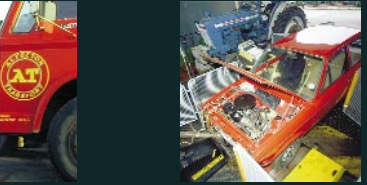
Ford Fiesta on rolling road
